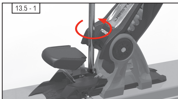
REPLACING THE SKI BRAKES DUKE PT, ROYAL FAMILY, FDT & TOUR:
